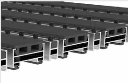
lastik + dar fırça rubber+narrow brush
